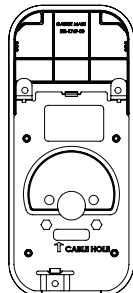
Mounting Plate
